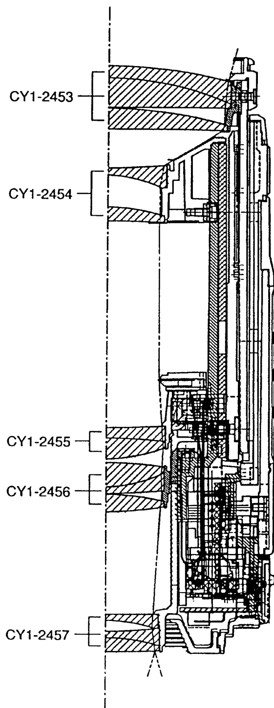
Fig. 13 Cross-section
